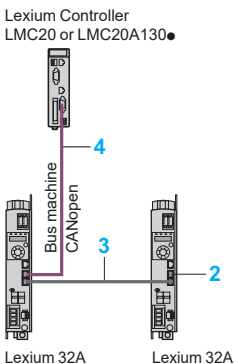
Example of architecture with control by Lexium Controller LMC
