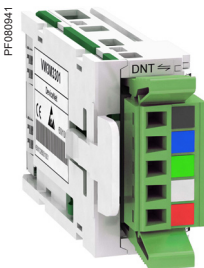
VW3M3301 DeviceNet communication card
